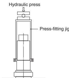
Fig. 6.1 Press-fitting pressure
