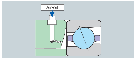
Fig. 9.21 79U and 70U types
