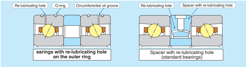
Fig. 9.34 HSEW Type
