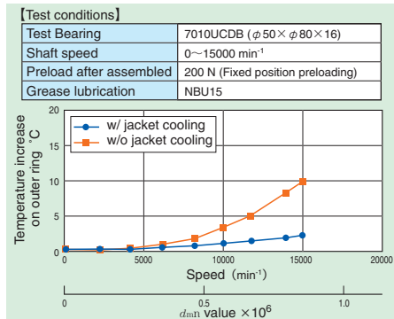
Fig. 9.22 High-speed test with grease lubrication
