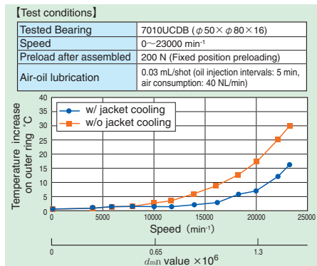
Fig. 9.23 High-speed test with air-oil lubrication
