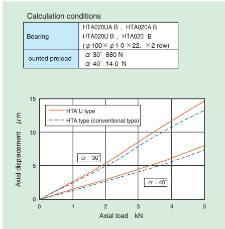
Fig. 11.3 Axial load and rigidity
