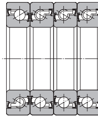
When three rows bear axial load (DBTT)
