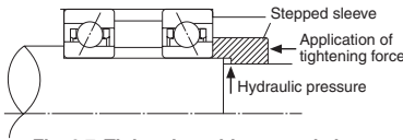
Fig. 6.7 Tightening with stepped sleeve
